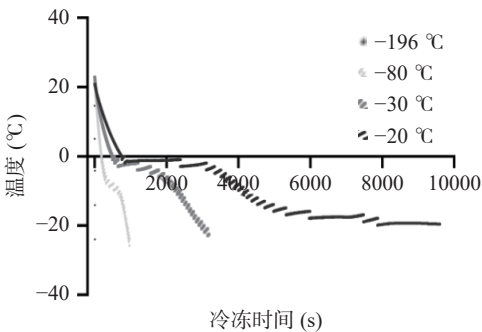
图 1 汤圆粉团在不同温度下的冷冻曲线 Fig.1 Freezing curve of rice dumpling dough at different temperatures
